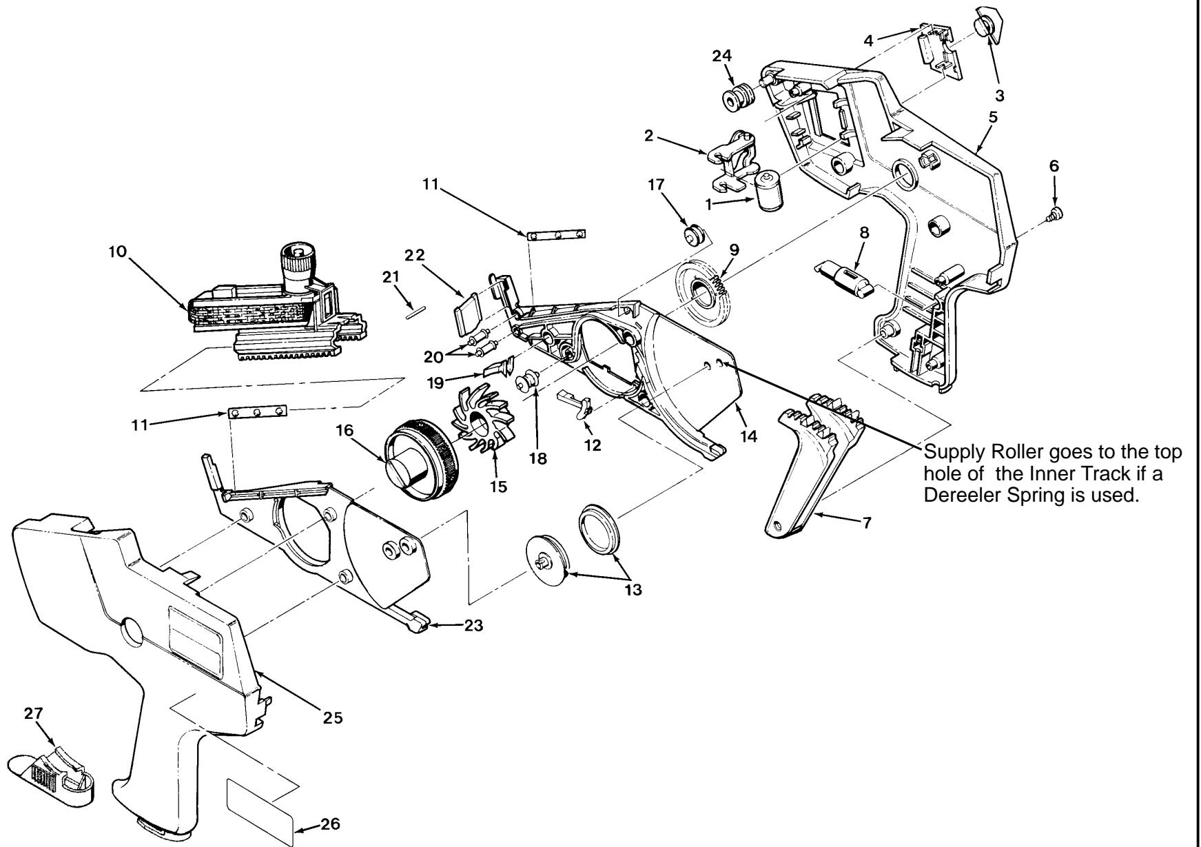
Figure 1. Labeler Assembly.
