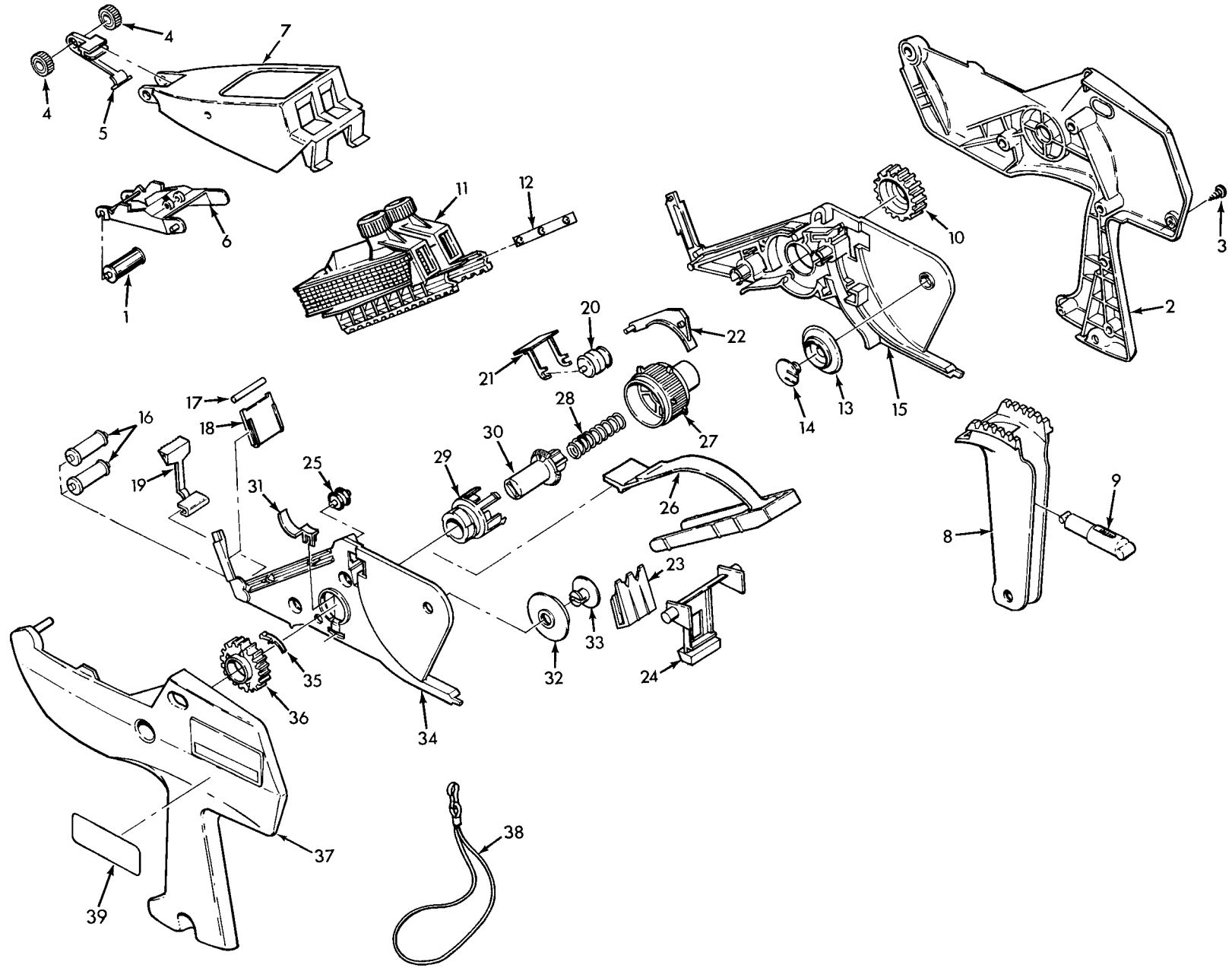
Figure 1. Labeler Assembly.
