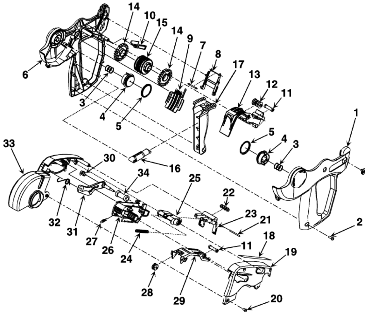
Figure 1. Labeler Assembly, 1 Line
